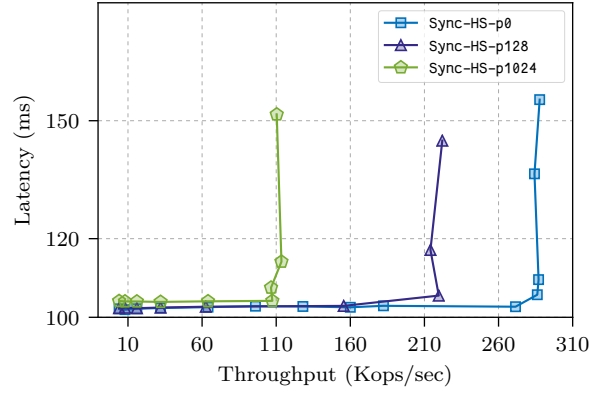
(b) Varying payload.
